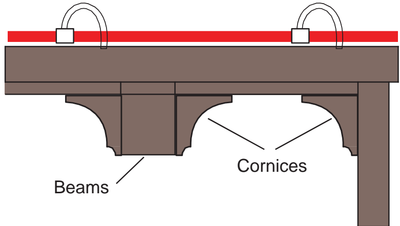
Capillary tubes runs above the ceiling and enter the fire zone through a small hole in the cornice
